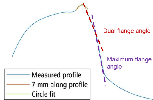
Calculation of minimum flange tip radius and flange angles
