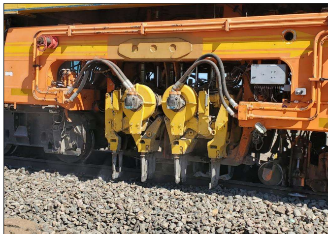
Tamper on Class 1 track
