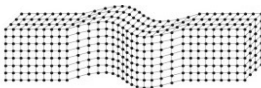
SH Waves
