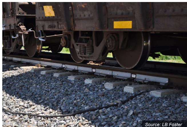
WILD site with lateral force (THD) sensors
