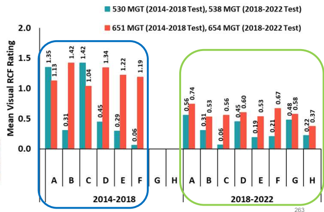
Mean visual RCF rating comparison, low rail for 2014 & 2018 tests
