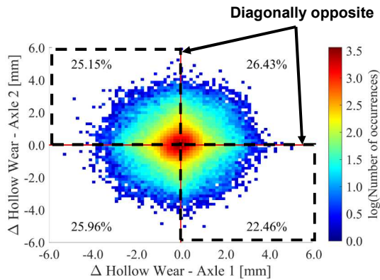
Comparison of hollow wear difference on Axles 1 and 2
