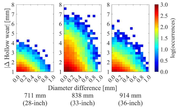
Hollow wear difference as a function of initial diameter difference
