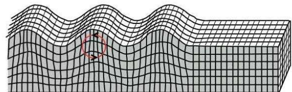
Surface Waves
