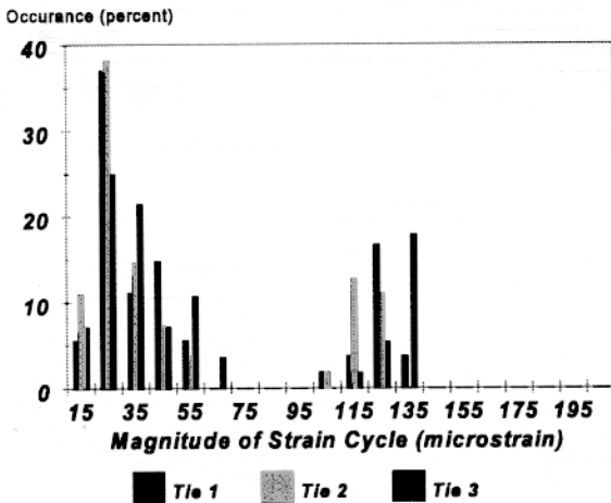
Exhibit 5. 33-Ton Axle Load-Distribution of Strain Cycles
