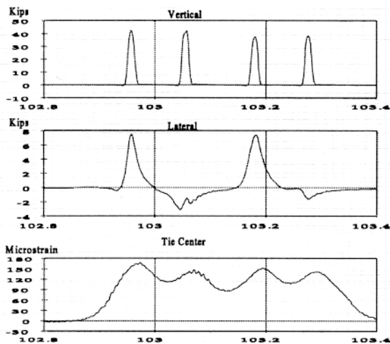
Exhibit 2. Vertical and Lateral Forces and Associated Strains - 39-Ton Axle Load Car
