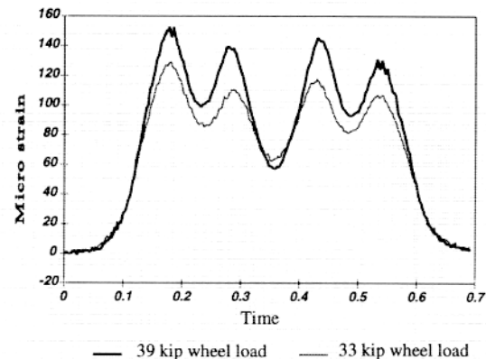
Exhibit 1. Typical Strain Response of 33- and 39-Ton Axle Load Cars
