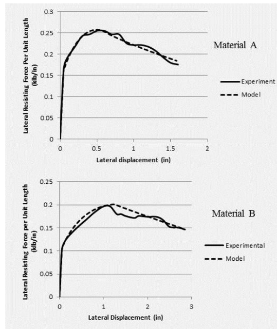
Figure 5. Model Prediction vs. Experiment for Two Representative Ballasts
