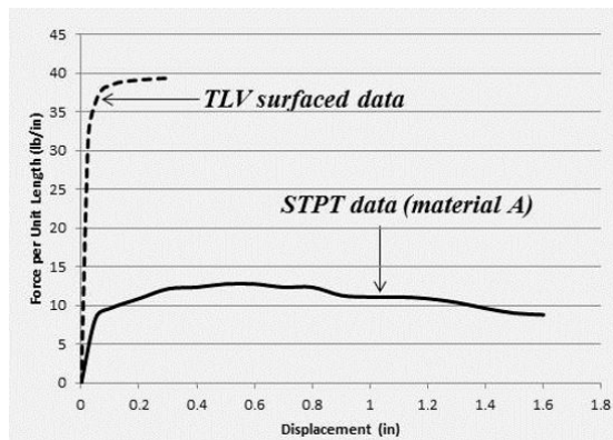
Figure 3. Comparison of Lateral Resistance Obtained from TLV and STPT Tests
