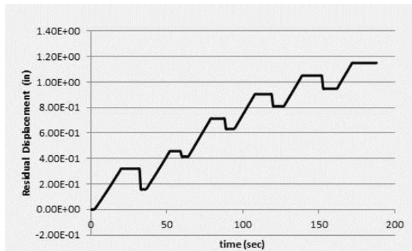
Figure 7. Predicted Evolution of Residual Displacement of the Rail Structure during Cyclic Loading
