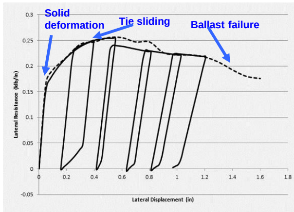
Figure 6. Predicted Lateral Resistance vs. Applied Lateral Displacement for Material A
