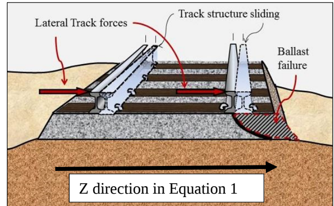
Figure 2. Schematic Depicting Deformation Mechanisms in Track Structure Due to Lateral Loading
