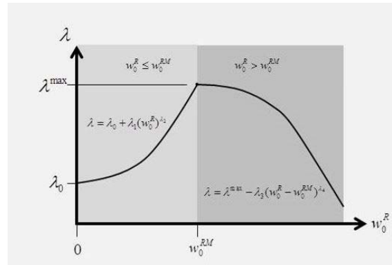
Figure 4. Schematic Depicting Method for Determining Nonlinear Lateral Resistance Coefficient ( \lambda(f_z) ) from a STPT Test
