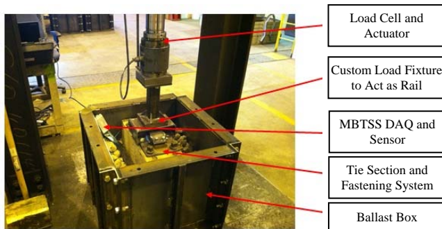
Figure 3. Laboratory Ballast Box Testing Configuration
