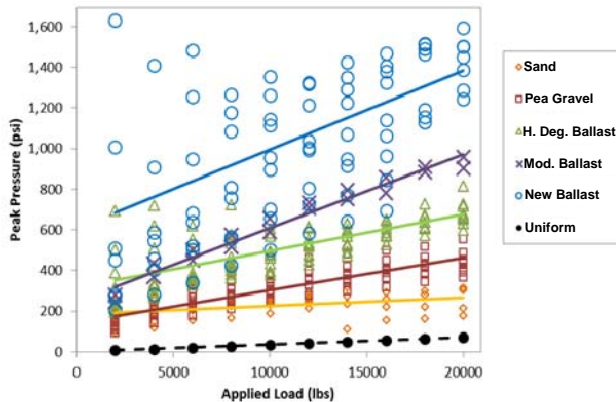
Figure 7. Peak Pressure vs. Applied Load for the Five Ballast Materials
