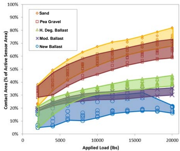
Figure 6. Contact Area vs. Applied Load for the Five Ballast Materials used in Laboratory Testing
