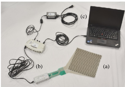
Figure 1. MBTSS System Components
