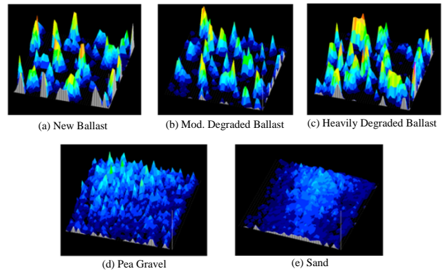
Figure 5. A Typical Pressure Distribution for Each of the Five Ballast Gradations
